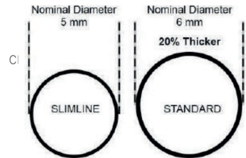
Cross Sectional Comparison between Slimline and Standard Patch Lead
