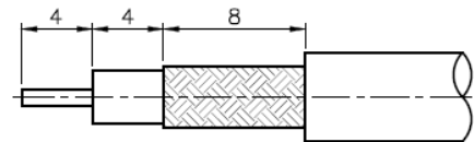
CABLE STRIPPING DIM'S
