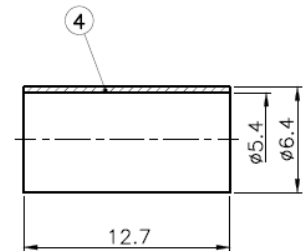
CABLE STRIPPING DIM'S
