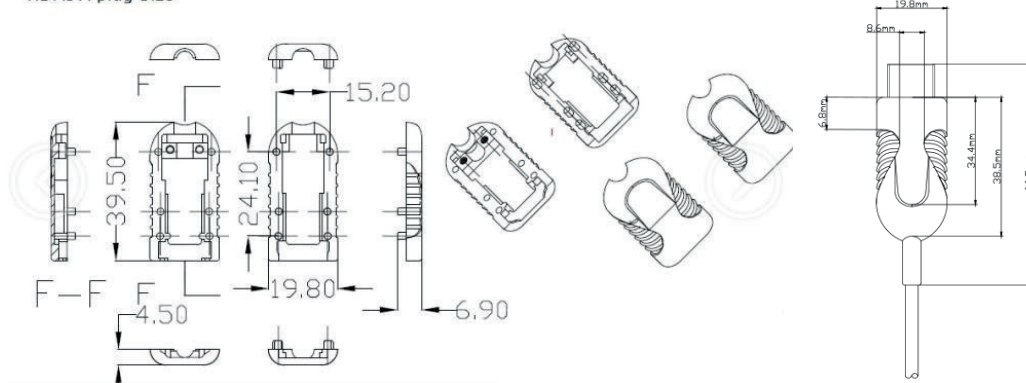
HDMI A plug Size
