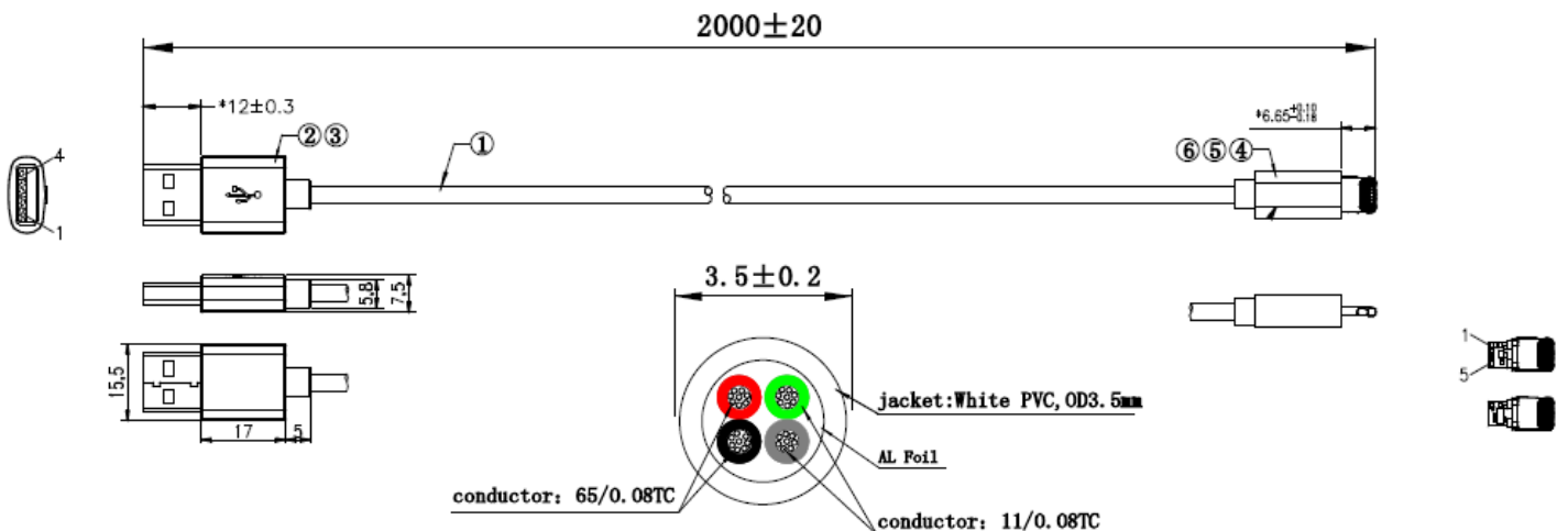
cable structure
