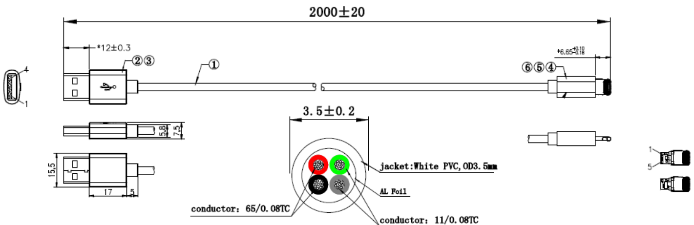
cable structure
